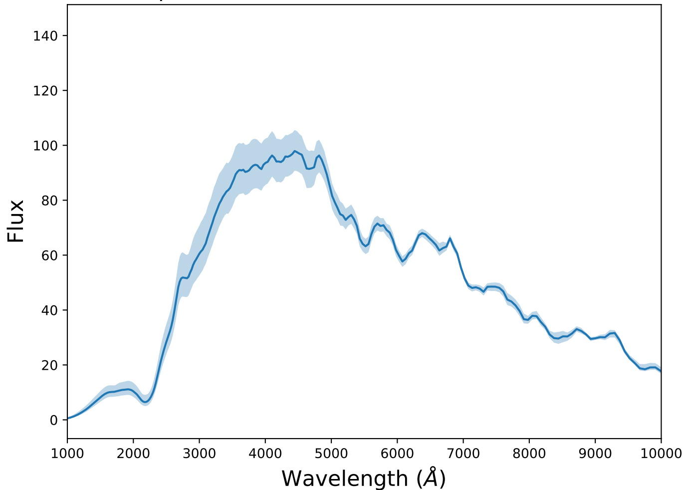
Spectrum 5 for transient CCSN at z=0.49
